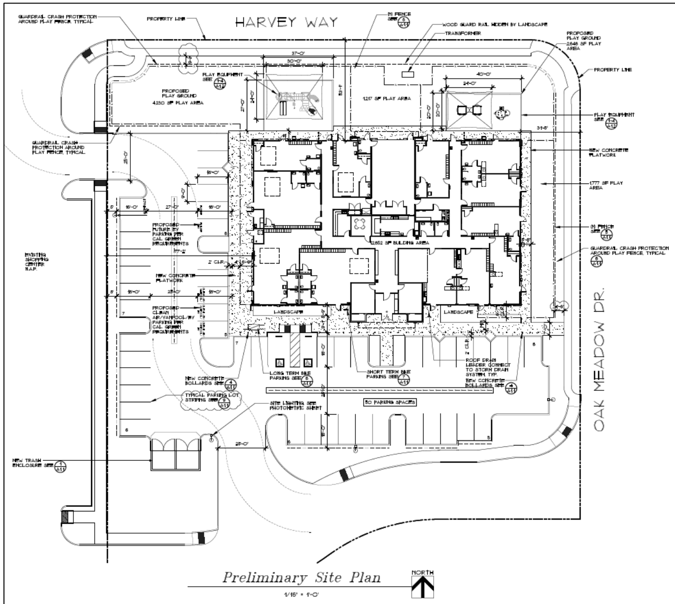
Figure 2: Site Plan
